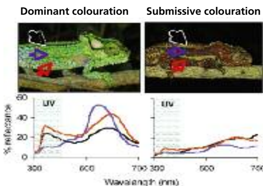
Measurements of chameleon colours revealed that several species, like the Knysna dwarf chameleon pictured here, use display colours with a UV component (peaks in the blue shaded region). Line colours correspond to the coloured arrows indicating the body regions measured.
